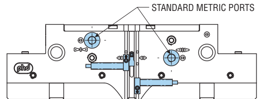
SIZES 92, 112, 133, 170 PROXIMITY SWITCH BRACKET MOUNTING LOCATIONS ON STANDARD UNITS WITH METRIC PORTS
