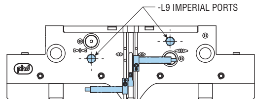
SIZES 92, 112, 133, 170 WITH -L9 IMPERIAL PORTS PROXIMITY SWITCH MOUNTING LOCATIONS
